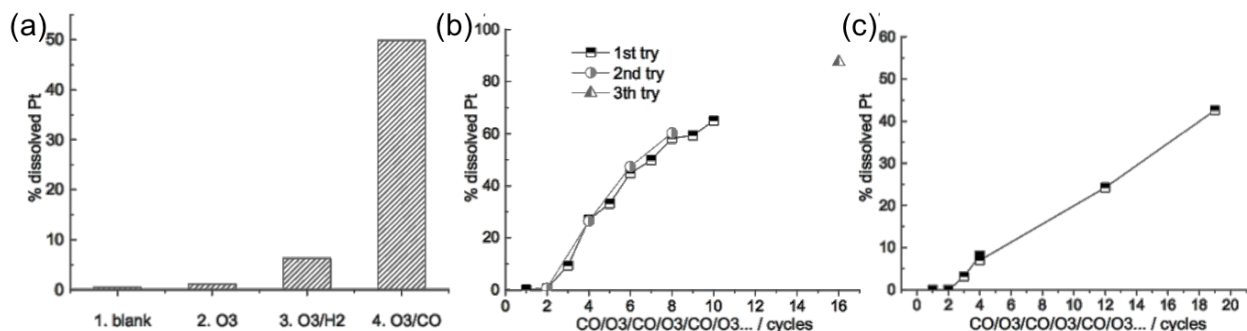
Fig.1: (a) Recycling of platinum from the platinum nanoparticles deposited on high surface area carbon (HSAC) with a 46% metal loading. The influence of presence of argon, O 3 , alternating O 3 /Ar/H 2 exposure and the alternating O 3 /Ar/CO in the mixture of 0.1 M HClO 4 and 0.1 M NaCl were investigated. HSACPt-containing material was drop casted as a thin film and dipped into the electrolyte solution, and rotated with 400 rpm. The diagram (a) shows the amount of the dissolved Pt (i) in the presence of Ar for 35 minutes, (ii) in the presence of O 3 for 35 minutes, (iii) in alternately presence of O 3 , Ar, O 2 , Ar, O 3 , Ar, H 2 , Ar, 5 minutes each cycle, (iv) in alternately presence of O 3 , Ar, CO, Ar, O 3 , Ar, CO, 5 minutes each cycle. The diagram (b) shows the amount of dissolved Pt obtained by stirring the HSAC Pt-containing material suspension exposure to: O 3 (20 min), Ar (10 min), CO (10 min), Ar (10 min), O 3 (10 min), Ar (5 min), Cl (10 min), Ar (10 min), O 3 (10 min), Ar (5 min) in 0.1 M HClO 4 . The diagram (c) shows the amount of dissolved Pt obtained by stirring the Car exhaust catalyst suspension exposure to: CO (20 min), Ar (5 min), O 3 (20 min), Ar (5 min), CO (20 min), Ar (5 min), O 3 (20 min), Ar (5 min) in 0.1 M HClO 4 .
