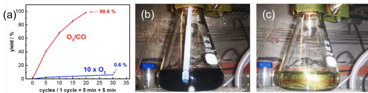
Fig. 2: (a) Pt Black powder suspension Pt yields of CO/ozone and pure ozone treatment in 0.3 M HCl + 1 M NaCl at room temperature. Images of before (b) and after (c) complete dissolution (yellow) of Pt suspension after 20 exchanges between ozone and CO.
